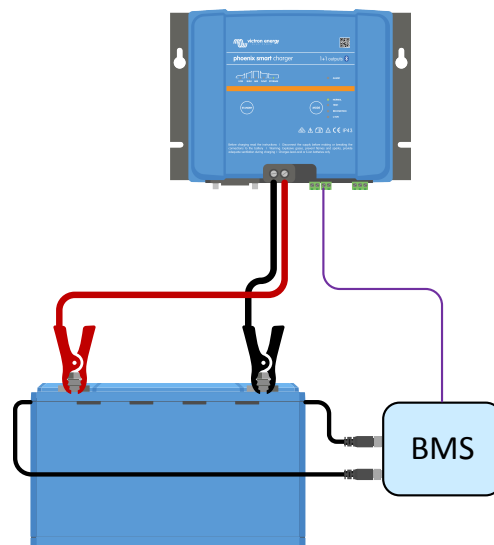
Initial charge using a BMS
